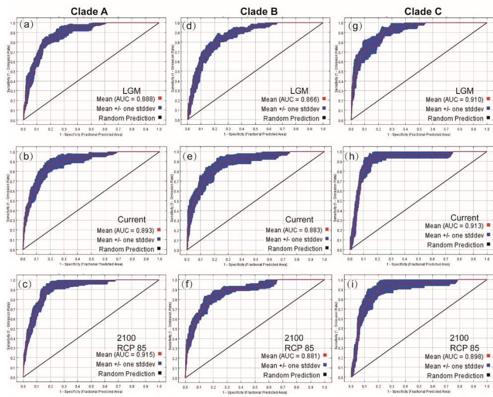
附录 6 核桃 3 个分支 Maxent 模型模拟结果模型精度统计。采用接收者操作特征曲线(receiver operator characteristic, ROC)和曲线下面积(areas under receiver operator characteristic curves, AUC)来共同进行评估。 Appendix 6 Statistical analysis of Maxent model accuracy simulation results from three Clades of Prunus mira . Evaluation is conducted jointly using receiver operator characteristic (ROC) and the areas under receiver operator characteristic curves (AUC).
