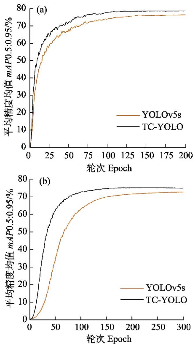
附录 3 数据集 Beijing-28 (a)与 CUB200-2011 (b)平均精度均值对比图 Appendix 3 The comparison chart of mAP between dataset Beijing-28 (a) and CUB200-2011 (b)
