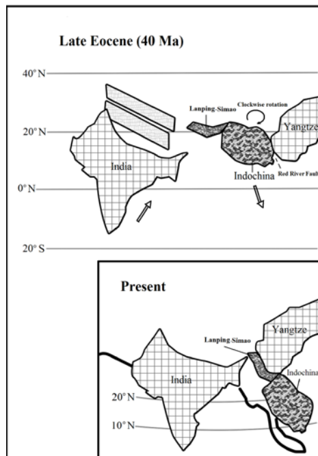
附录2 始新世晚期兰坪-思茅和印度支那板块顺时针转动及向东南逃逸示意图(引自Sato K, Liu YY, Zhu ZC, Yang ZY, Otofujii YI (2001) Tertiary paleomagnetic data from northwestern Yunnan, China: Further evidence for large clockwise rotation of the Indochina Block and its tectonic implications. Earth and Planetary Science Letters , 185, 185–198.)
