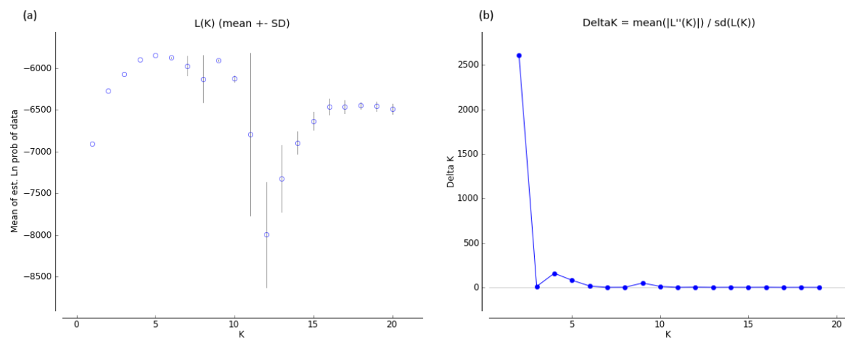
附录3 扁核木32个种群STRUCTURE分析中后验概率[ \ln P(D) ] (a)和后验概率的变化速率( \Delta K ) (b)分布 Appendix 3 Distribution of the change in log-likelihood of the data for each run, \ln P(D) (a), and \Delta K , the second order rate of change of \ln P(D) between successive K -values (b) in STRUCTURE analysis of 32 populations of Prinsepia utilis
