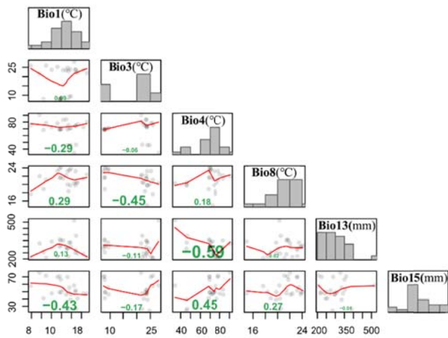
6 附录2 方差膨胀因子小于10的环境变量间的相关系数矩阵 8 Appendix 2 Correlation coefficient matrix between environmental variables with variance inflation factor value less than 10
